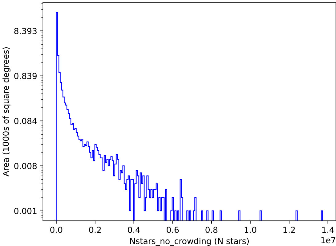
baseline_v2.1_10yrs g: Nstars_no_crowding
