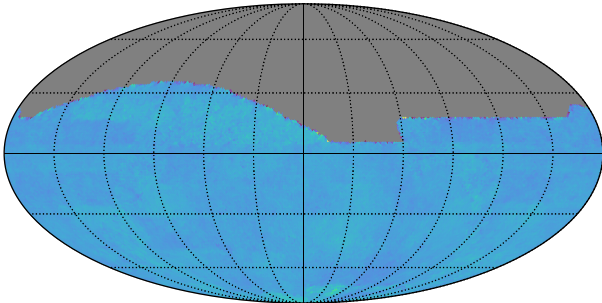
baseline_v2.1_10yrs : Normalized Proper Motion Uncert @ 24.0
