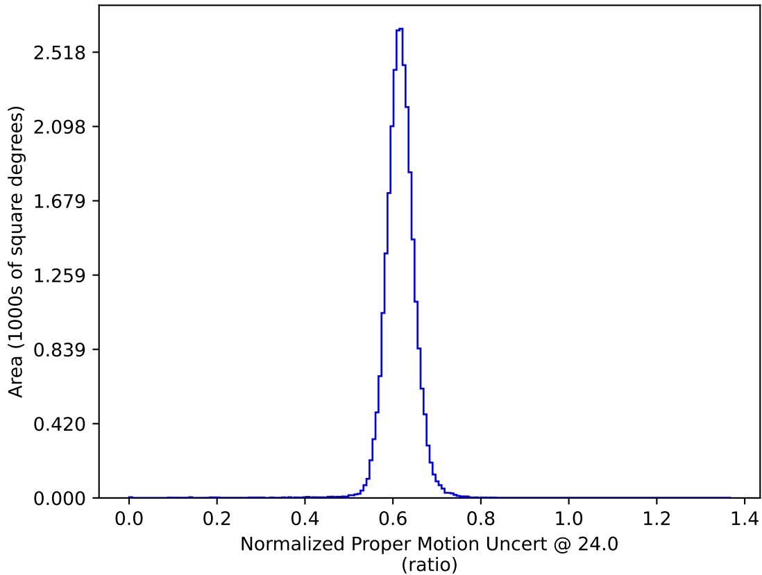
baseline_v2.1_10yrs : Normalized Proper Motion Uncert @ 24.0
