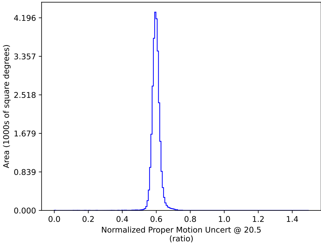
baseline_v2.1_10yrs : Normalized Proper Motion Uncert @ 20.5
