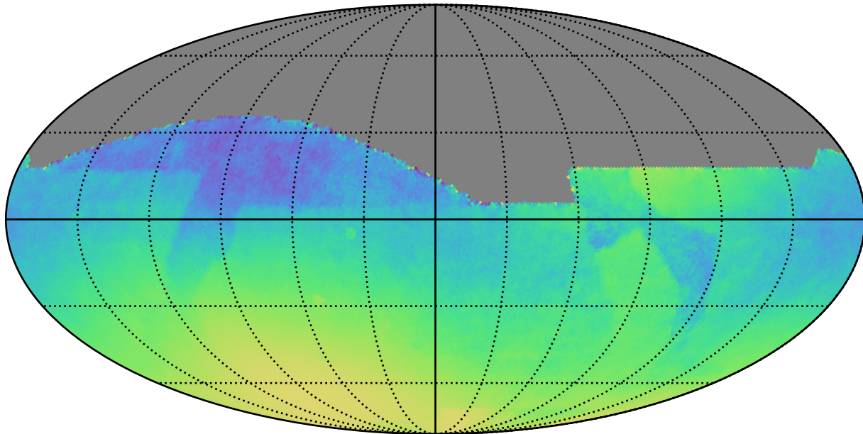
baseline_v2.1_10yrs : Normalized Parallax Uncert @ 24.0
