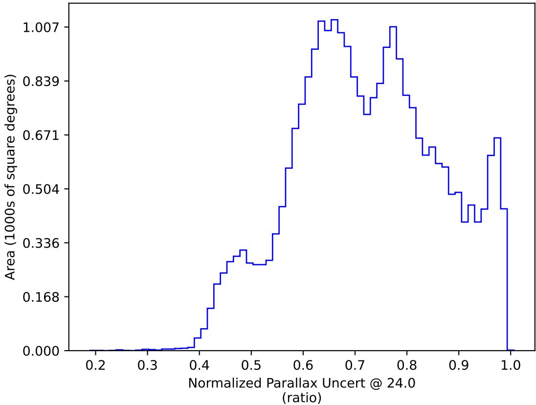
baseline_v2.1_10yrs : Normalized Parallax Uncert @ 24.0
