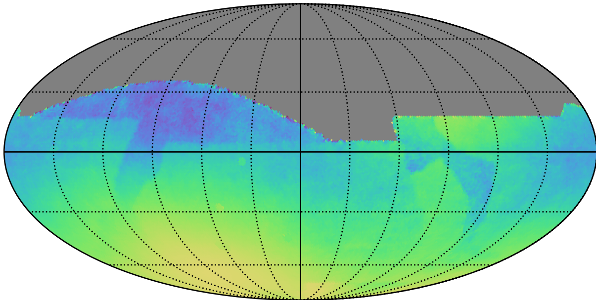
baseline_v2.1_10yrs : Normalized Parallax Uncert @ 22.4
