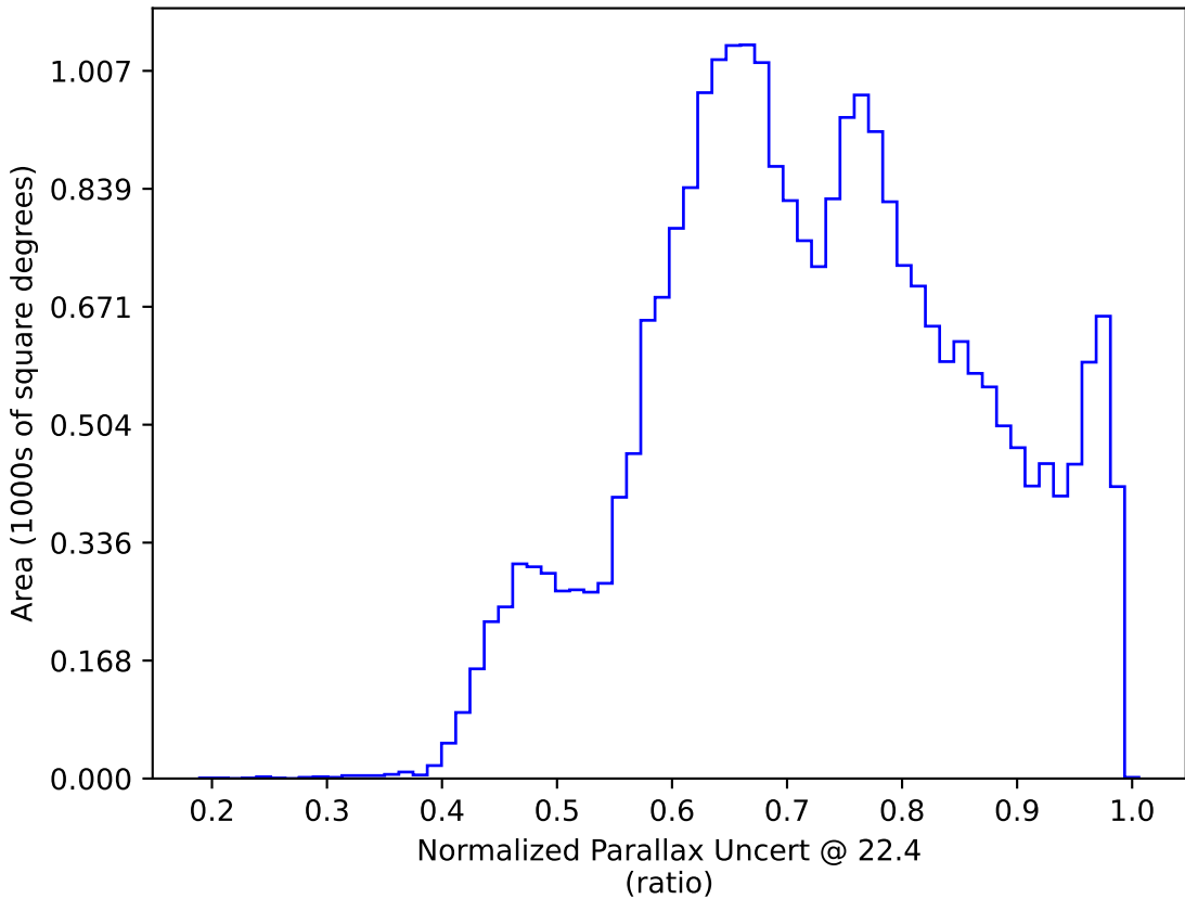
baseline_v2.1_10yrs : Normalized Parallax Uncert @ 22.4
