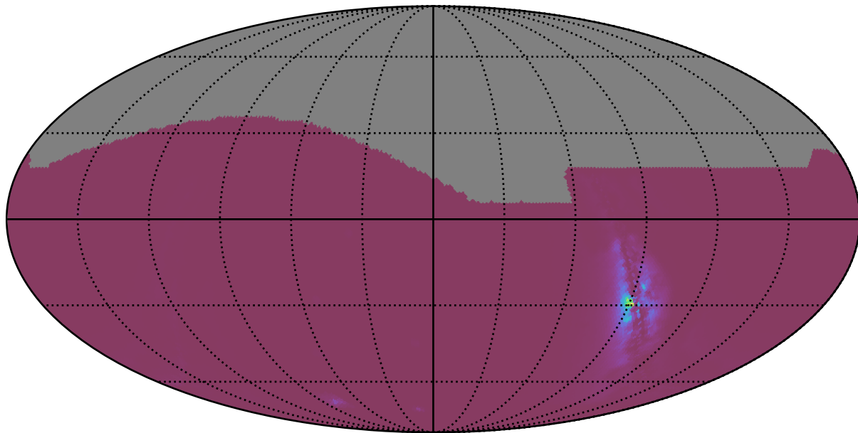
baseline_v2.1_10yrs : NlcPoints
