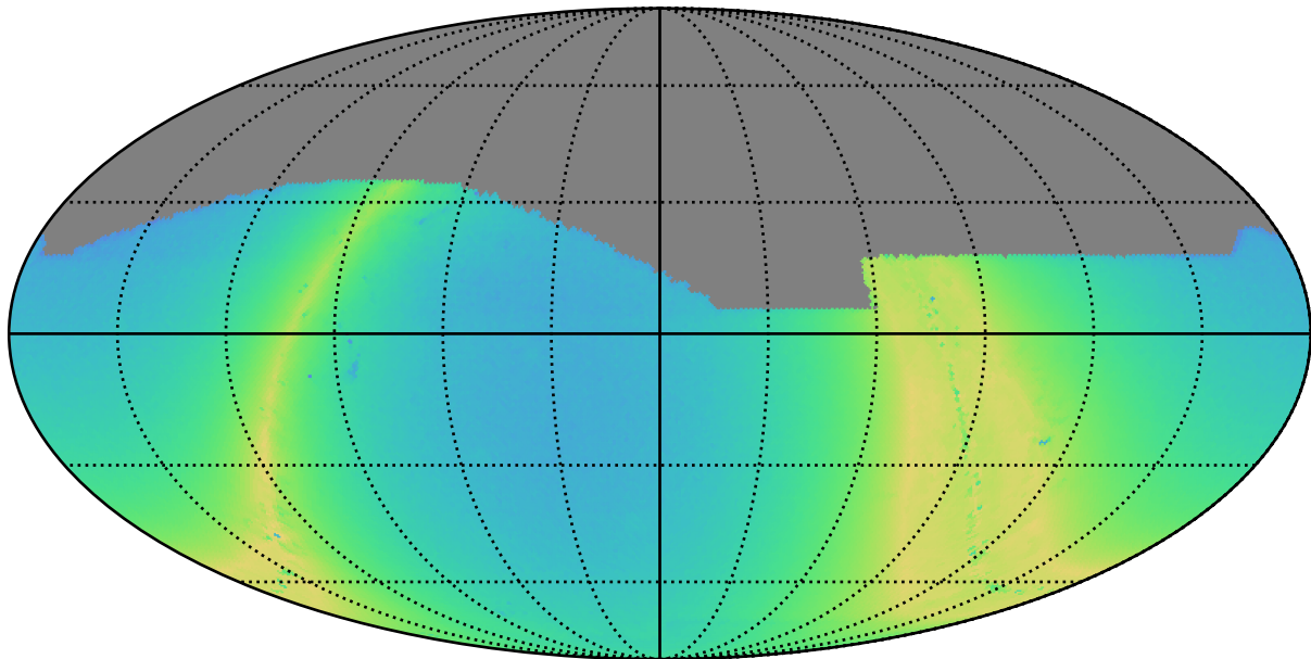
baseline_v2.1_10yrs z: N stars to Precision 0.20
