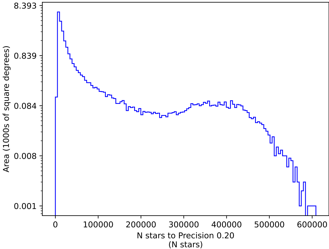
baseline_v2.1_10yrs z: N stars to Precision 0.20
