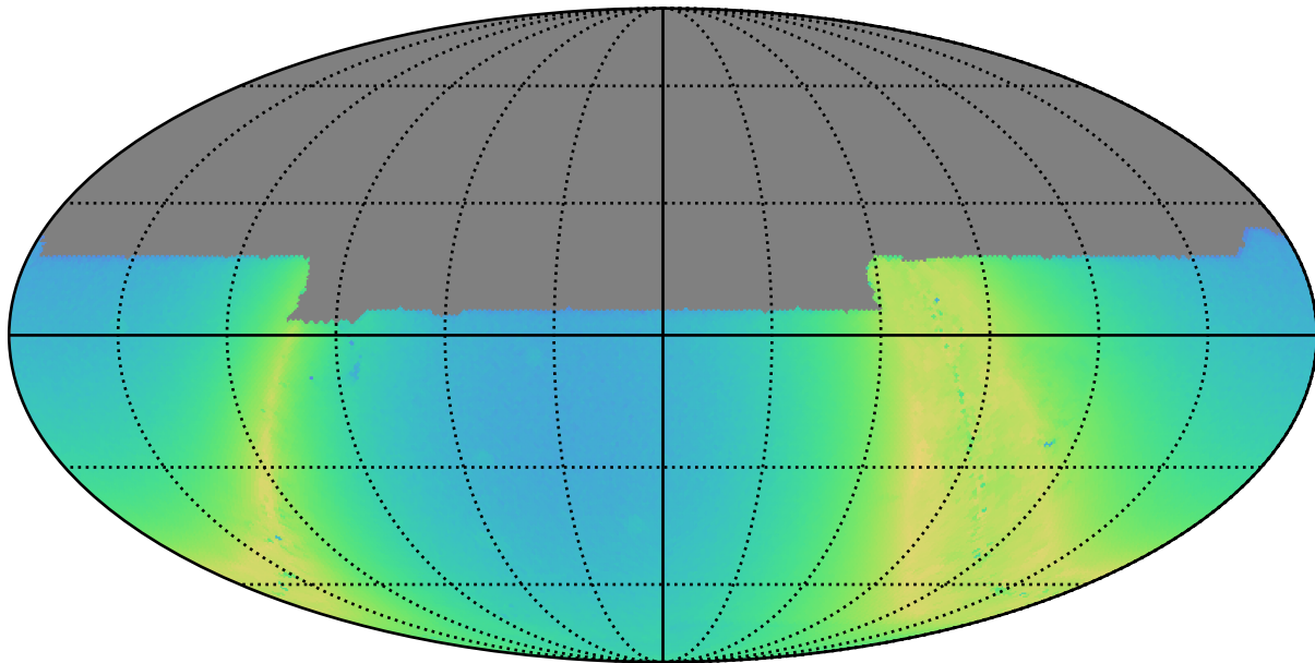
baseline_v2.1_10yrs y: N stars to Precision 0.20
