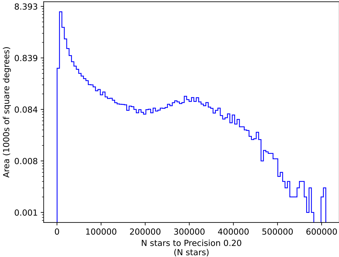
baseline_v2.1_10yrs y: N stars to Precision 0.20
