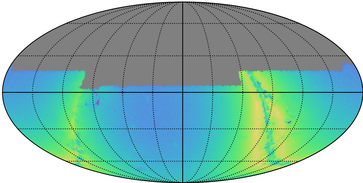
baseline_v2.1_10yrs u: N stars to Precision 0.20
