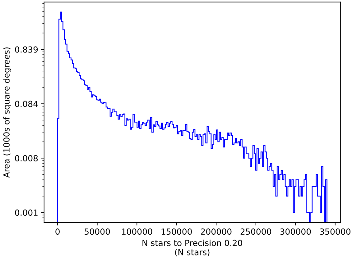
baseline_v2.1_10yrs u: N stars to Precision 0.20
