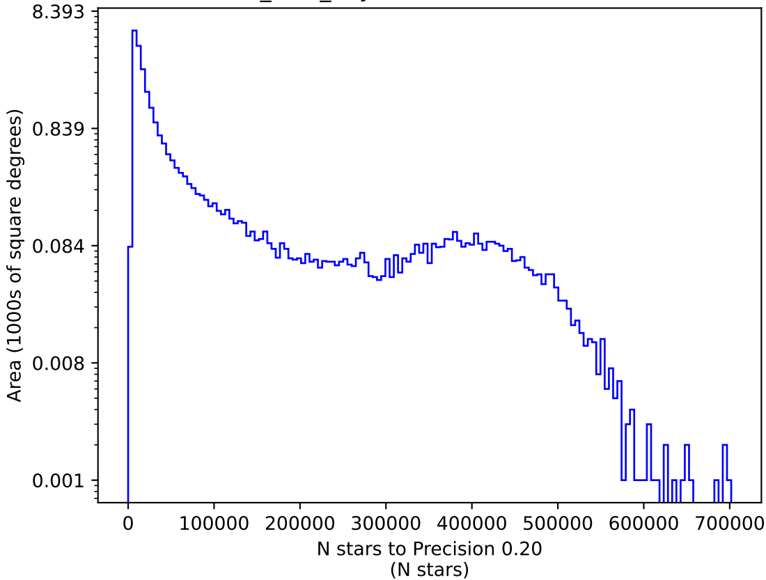
baseline_v2.1_10yrs i: N stars to Precision 0.20
