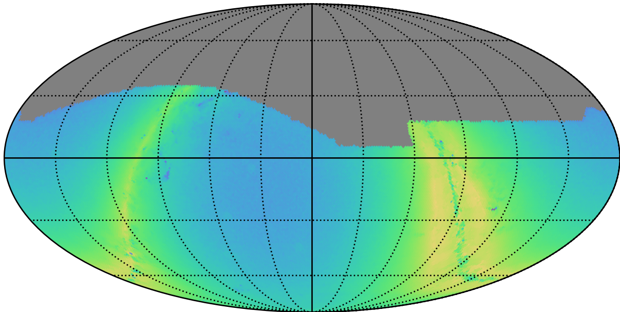
baseline_v2.1_10yrs g: N stars to Precision 0.20
