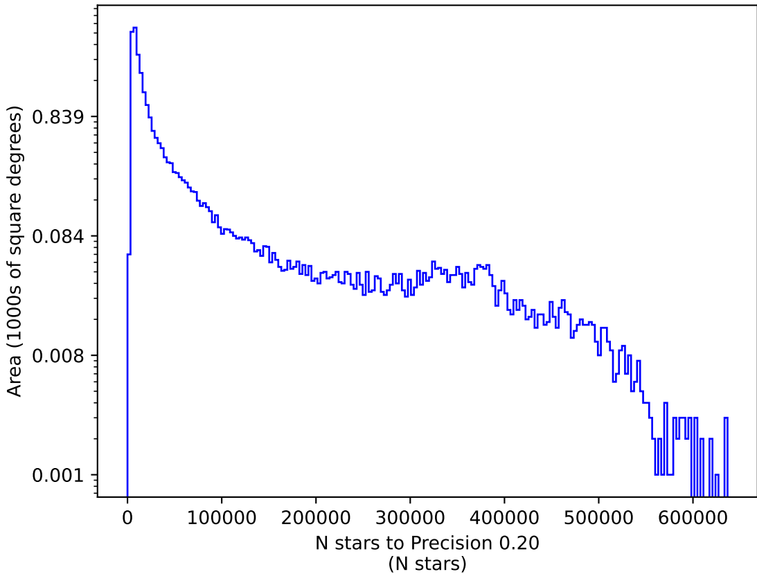
baseline_v2.1_10yrs g: N stars to Precision 0.20
