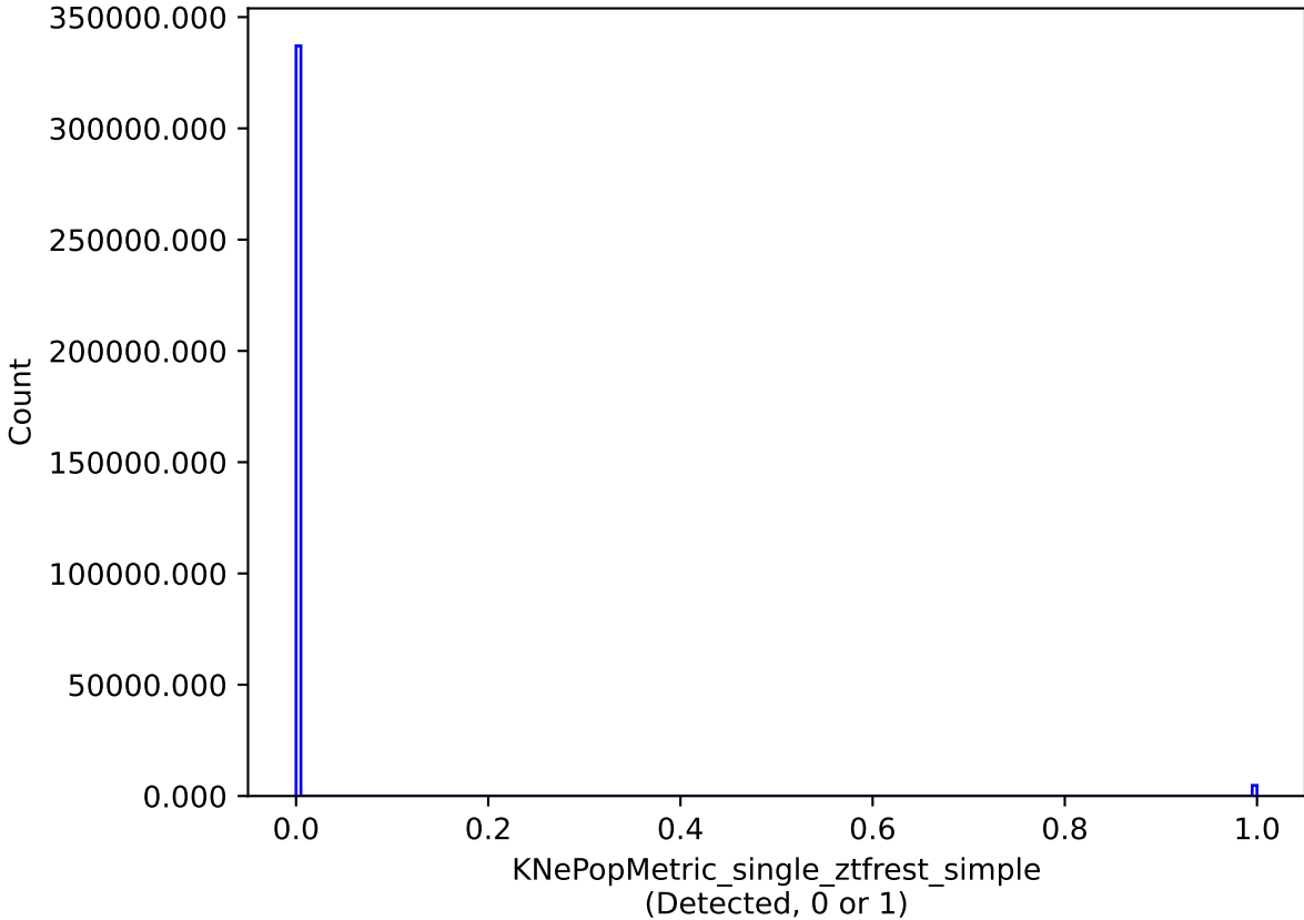
baseline_v2.1_10yrs single model: KNePopMetric_single_ztfrest_simple
