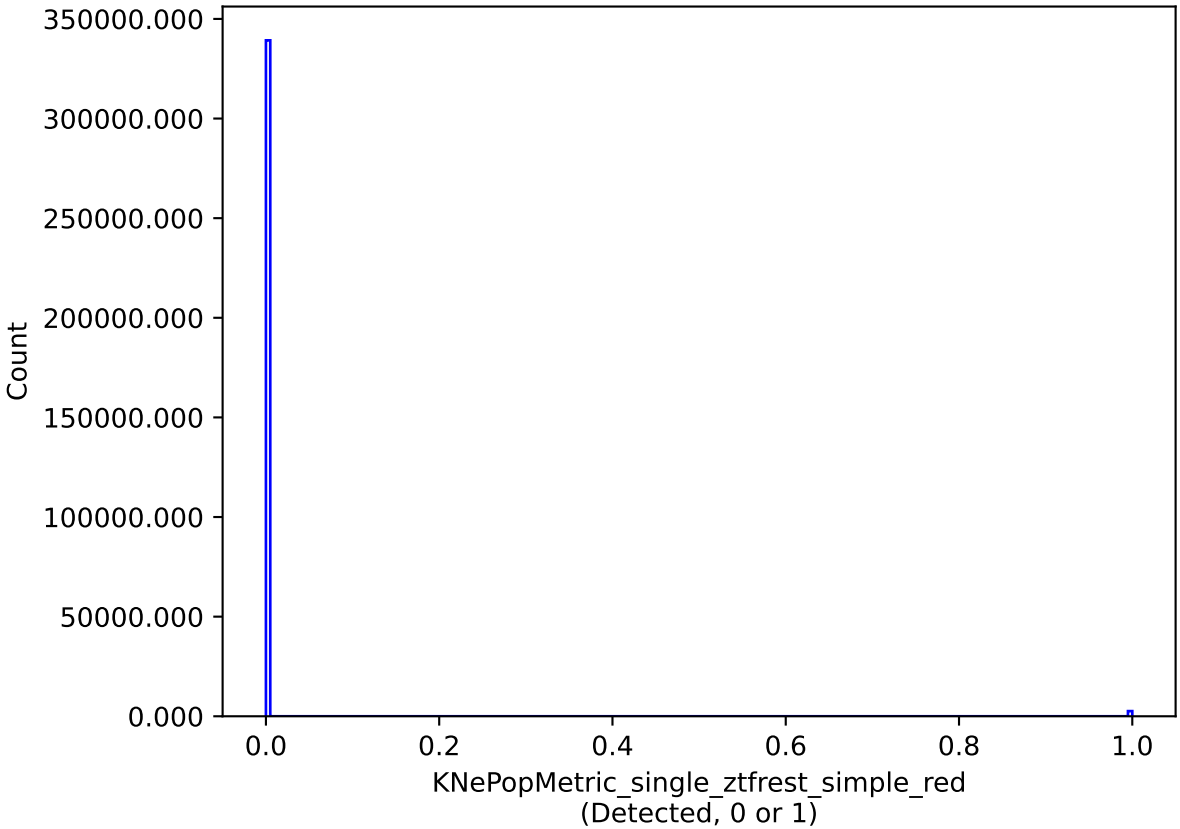
baseline_v2.1_10yrs single model: KNePopMetric_single_ztfrest_simple_red
