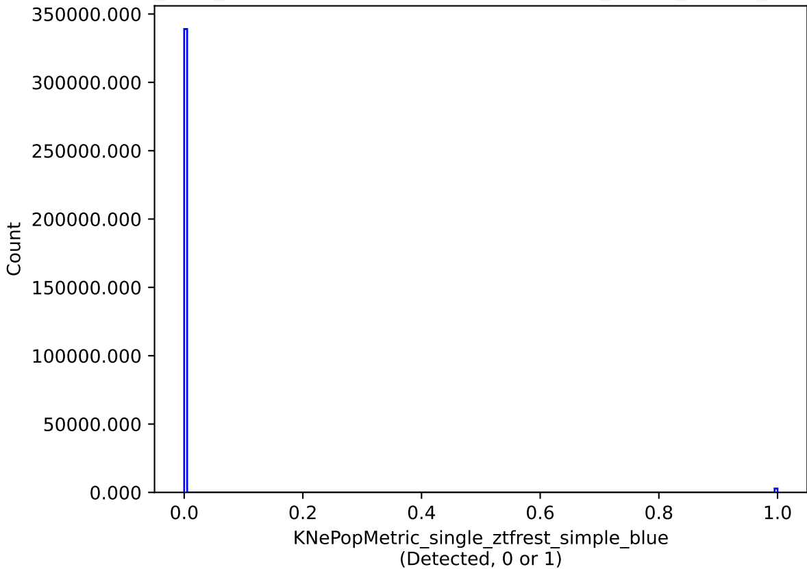
baseline_v2.1_10yrs single model: KNePopMetric_single_ztfrest_simple_blue
