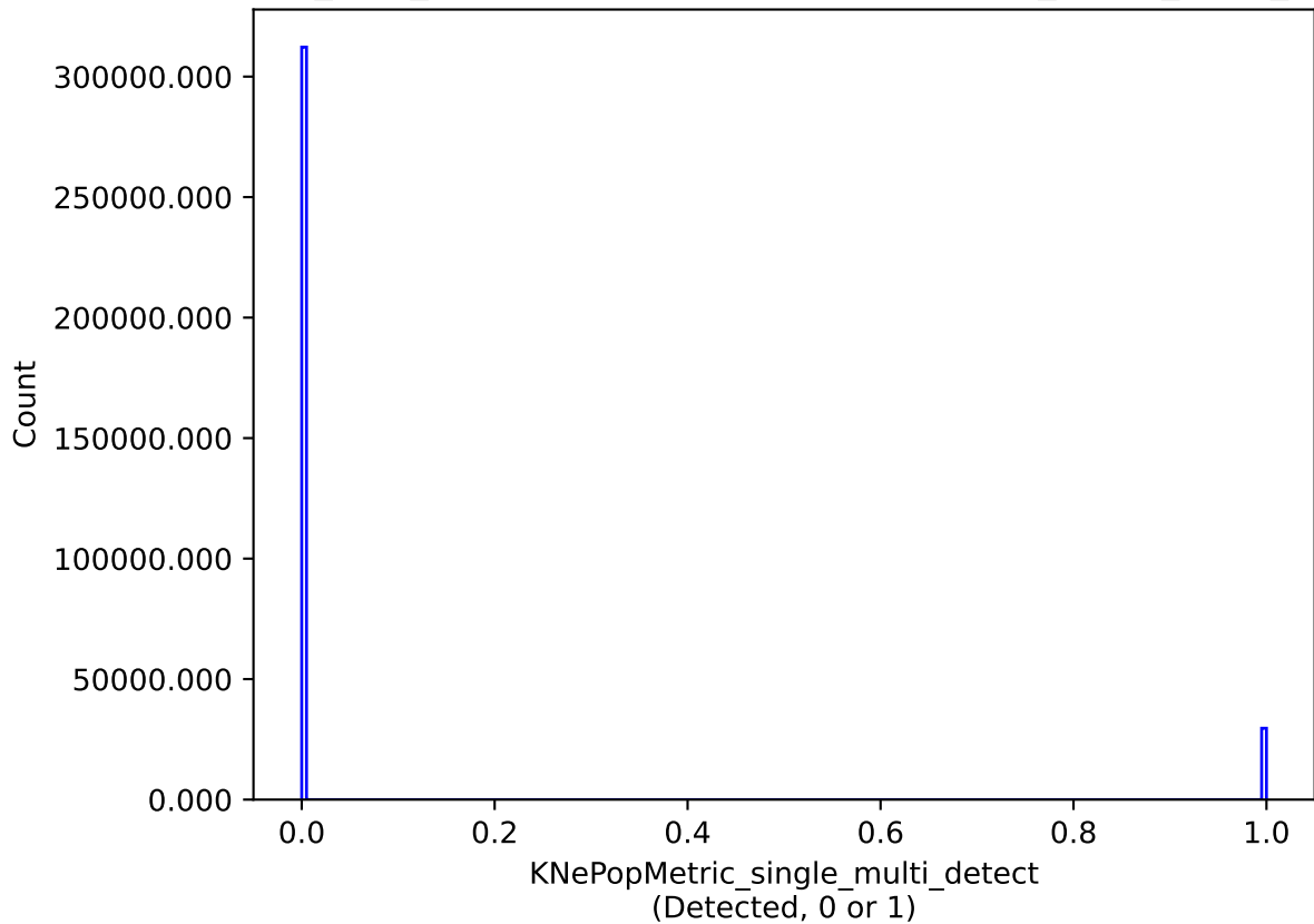
baseline_v2.1_10yrs single model: KNePopMetric_single_multi_detect
