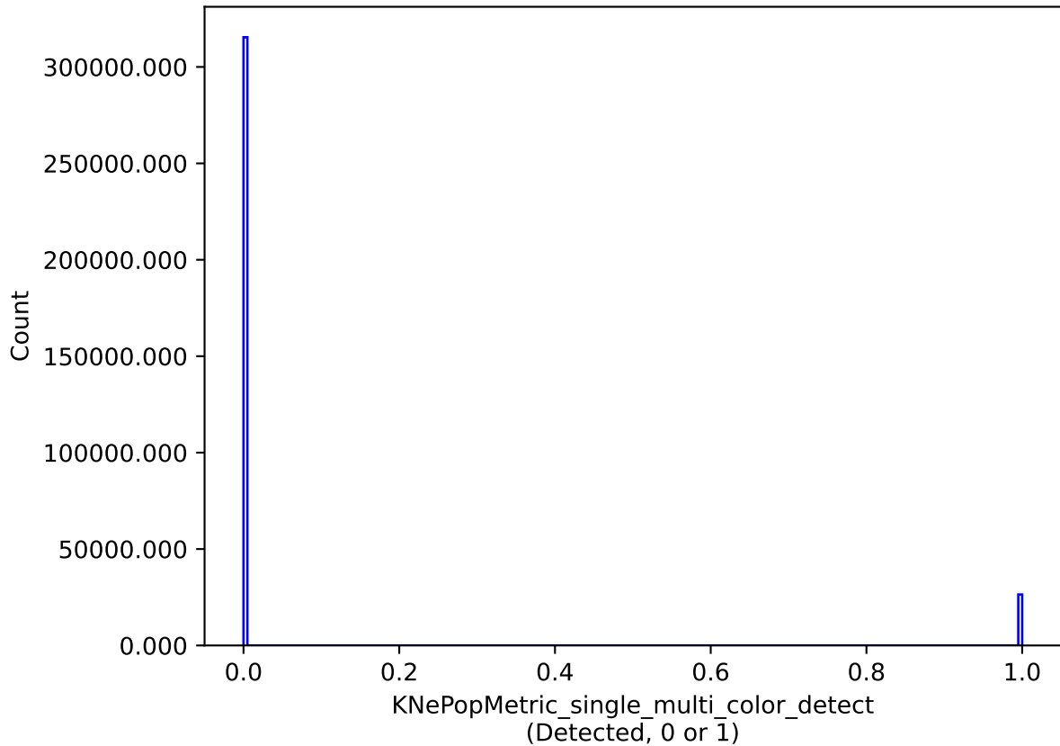
baseline_v2.1_10yrs single model: KNePopMetric_single_multi_color_detect
