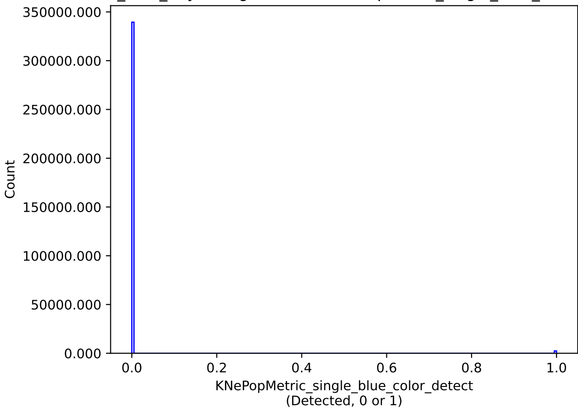
baseline_v2.1_10yrs single model: KNePopMetric_single_blue_color_detect
