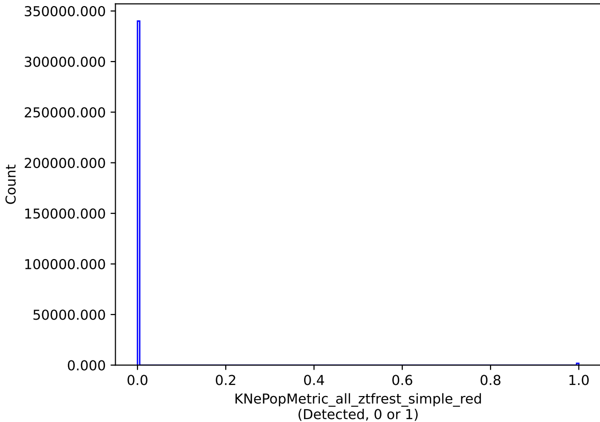
baseline_v2.1_10yrs all models: KNePopMetric_all_ztfrest_simple_red
