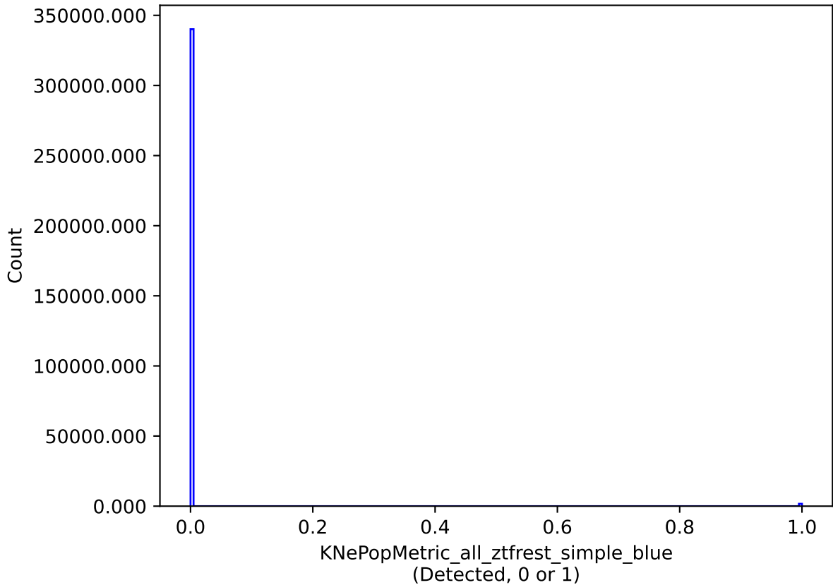
baseline_v2.1_10yrs all models: KNePopMetric_all_ztfrest_simple_blue
