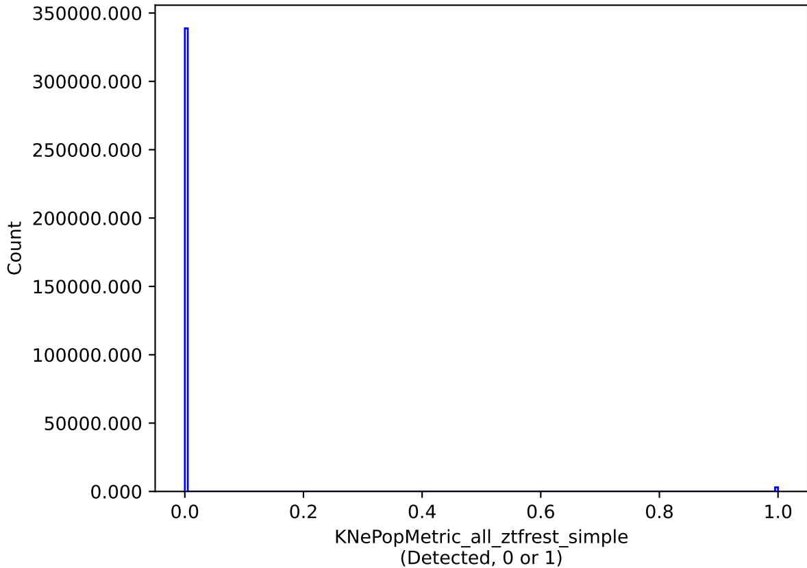
baseline_v2.1_10yrs all models: KNePopMetric_all_ztfrest_simple
