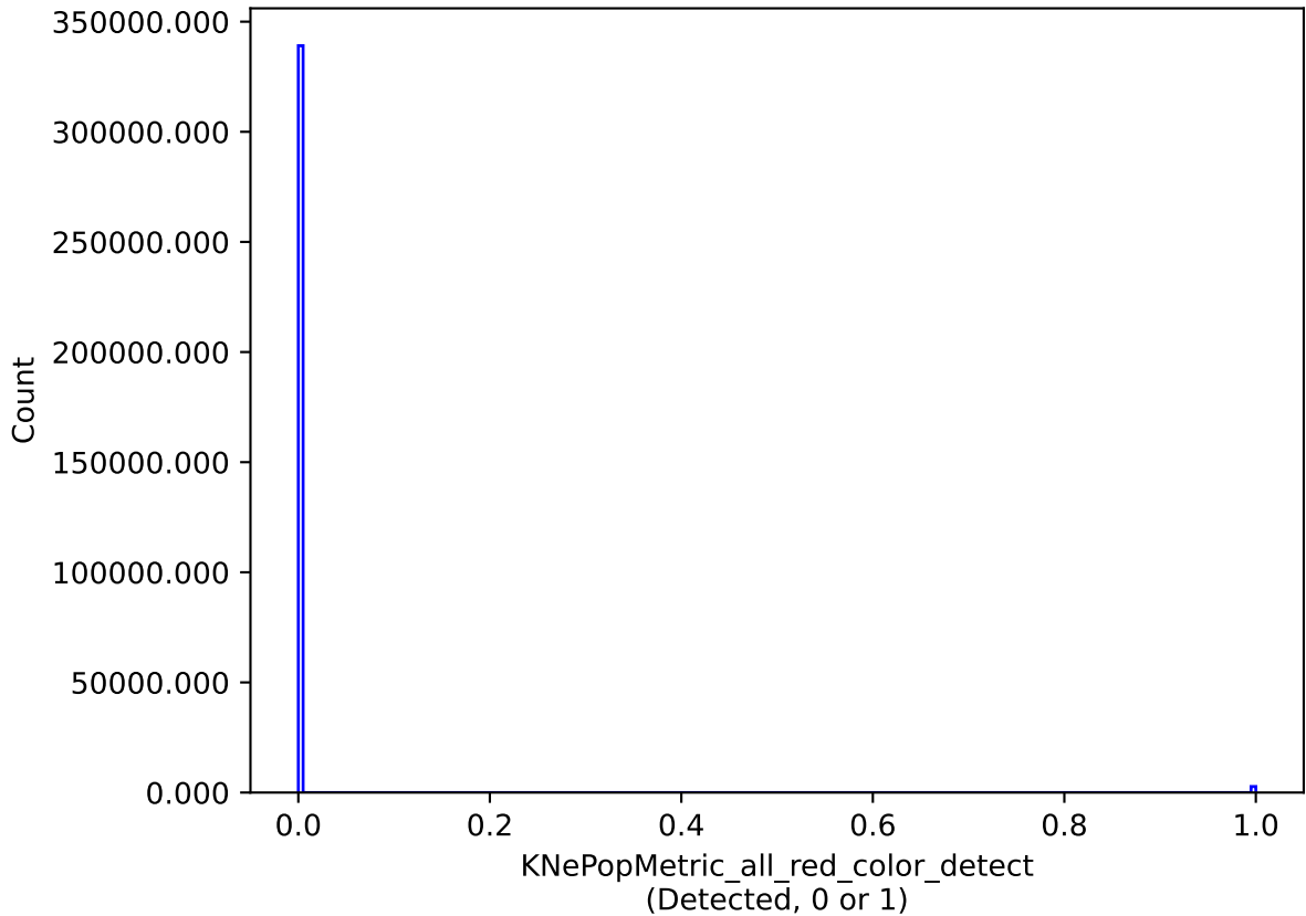
baseline_v2.1_10yrs all models: KNePopMetric_all_red_color_detect
