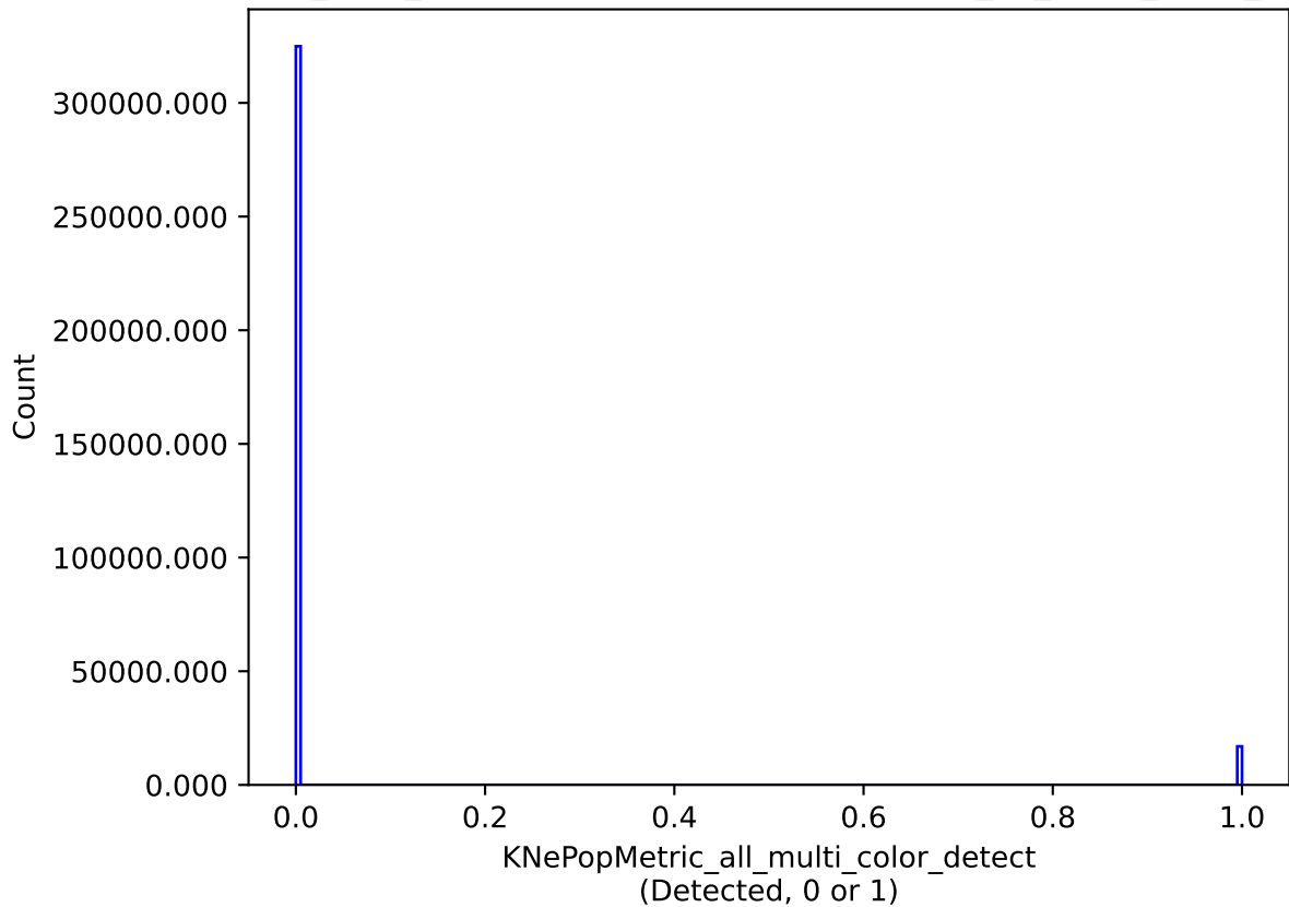
baseline_v2.1_10yrs all models: KNePopMetric_all_multi_color_detect
