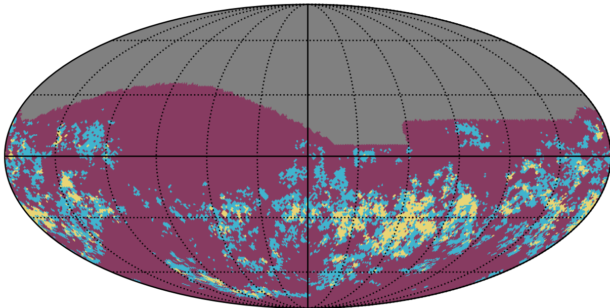
baseline_v2.1_10yrs z band: Gaps_7hr
