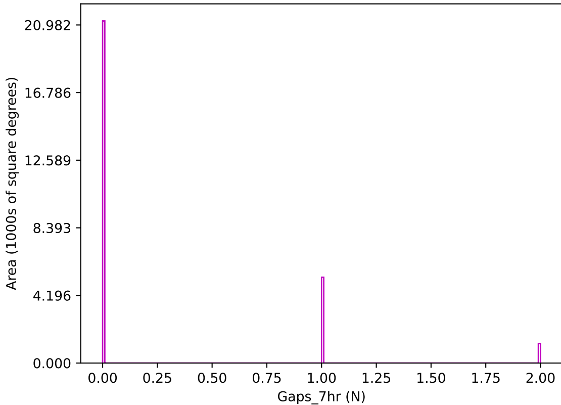
baseline_v2.1_10yrs z band: Gaps_7hr
