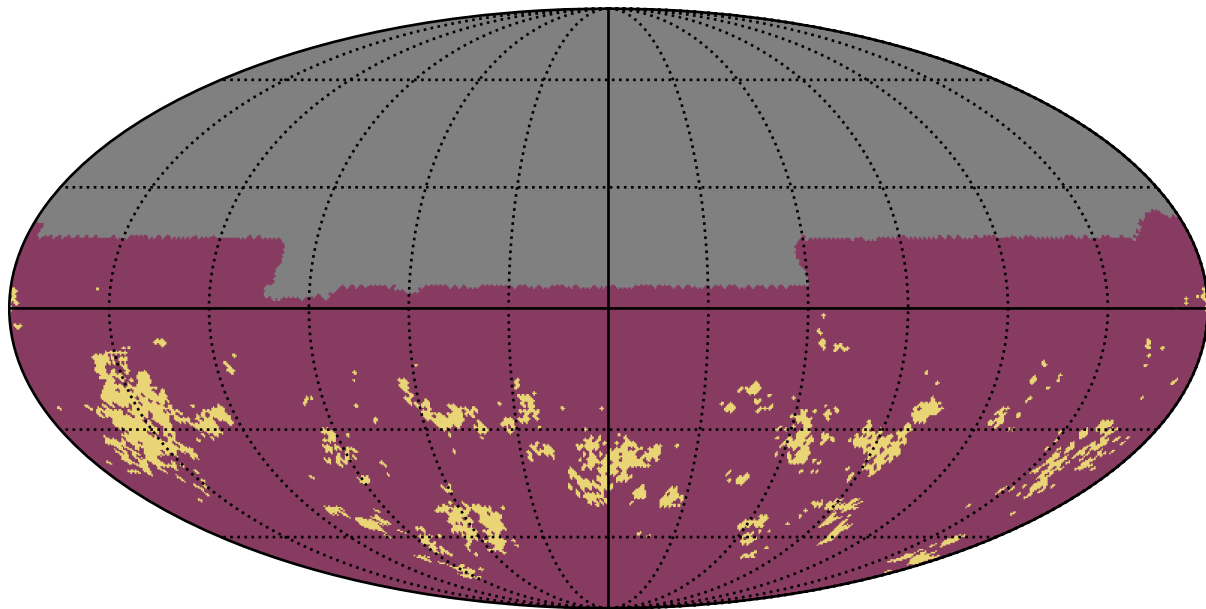
baseline_v2.1_10yrs u band: Gaps_7hr
