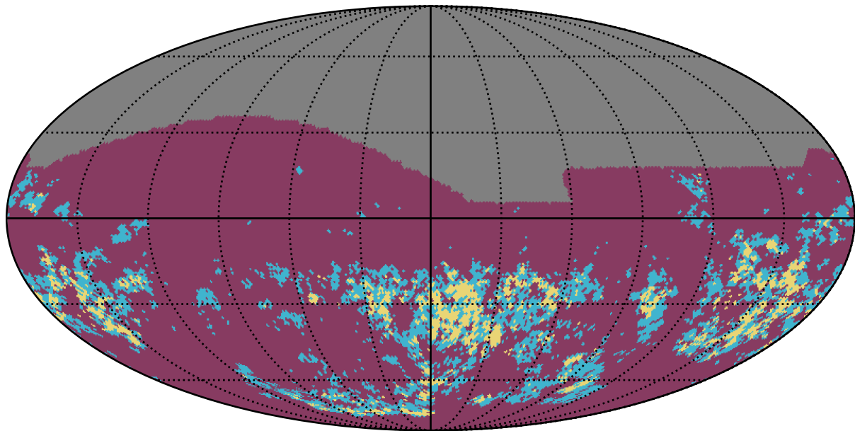
baseline_v2.1_10yrs r band: Gaps_7hr
