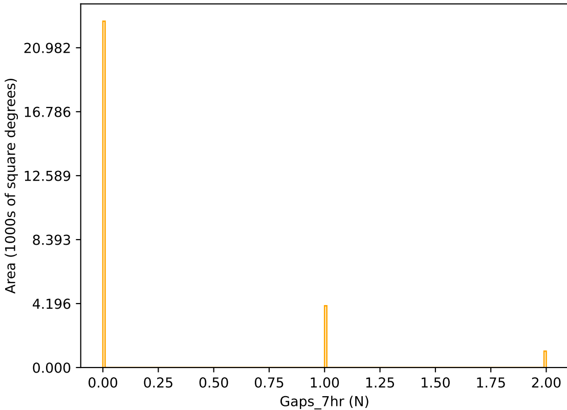
baseline_v2.1_10yrs r band: Gaps_7hr
