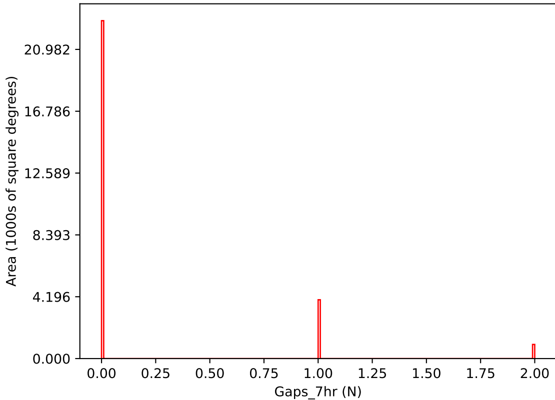
baseline_v2.1_10yrs i band: Gaps_7hr
