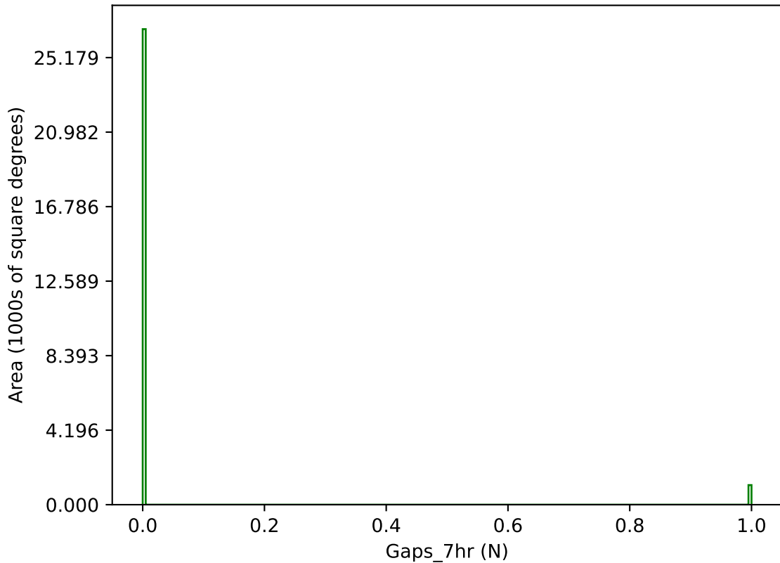
baseline_v2.1_10yrs g band: Gaps_7hr
