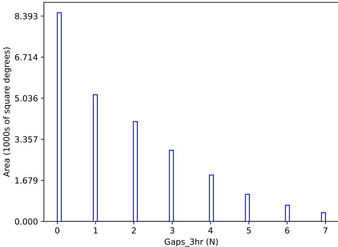
baseline_v2.1_10yrs y band: Gaps_3hr
