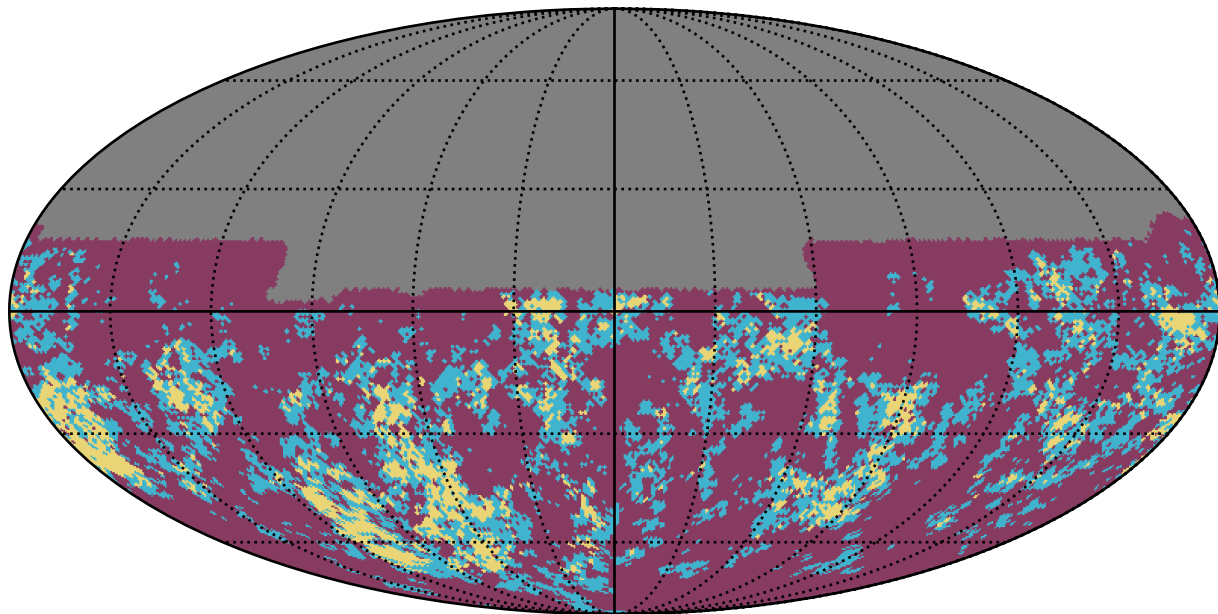
baseline_v2.1_10yrs u band: Gaps_3hr
