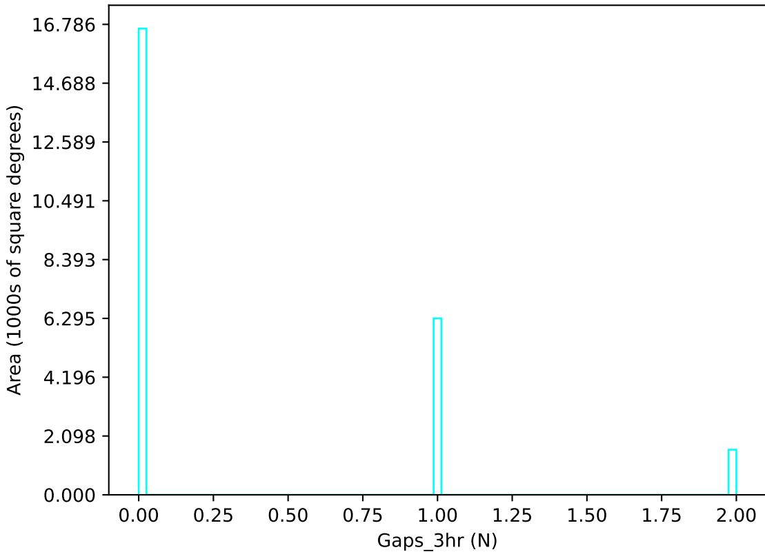
baseline_v2.1_10yrs u band: Gaps_3hr
