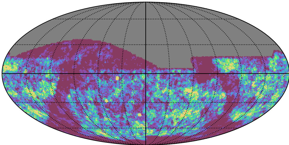
baseline_v2.1_10yrs r band: Gaps_3hr
