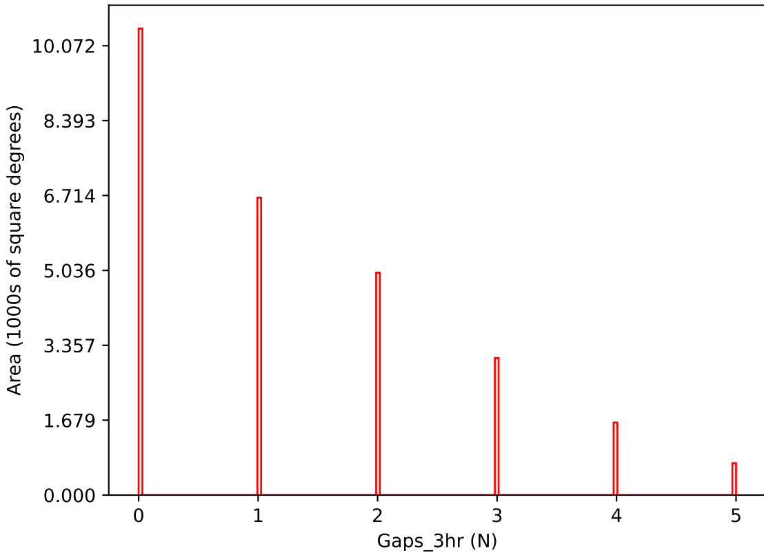
baseline_v2.1_10yrs i band: Gaps_3hr
