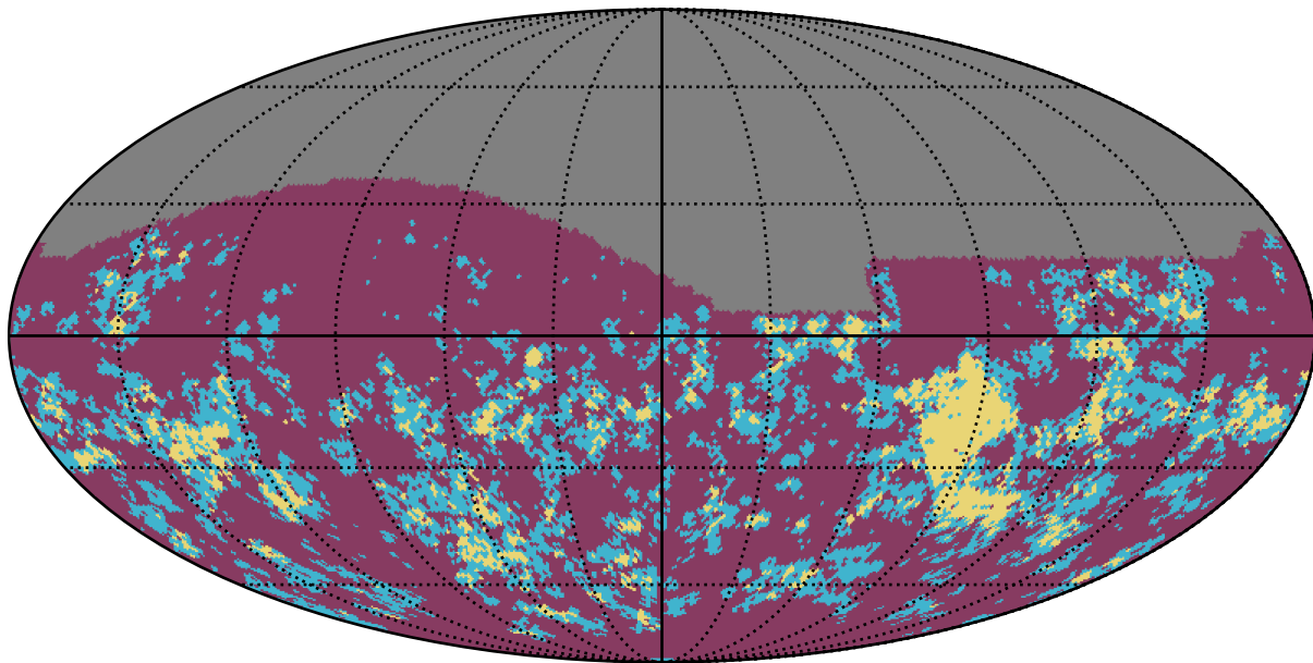
baseline_v2.1_10yrs g band: Gaps_3hr
