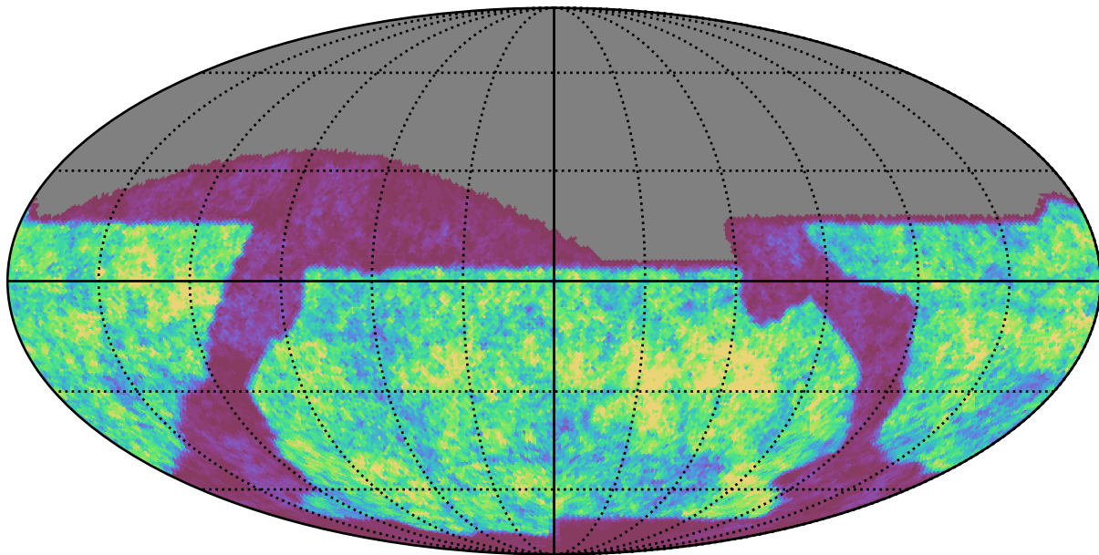
baseline_v2.1_10yrs z band: Gaps_24hr
