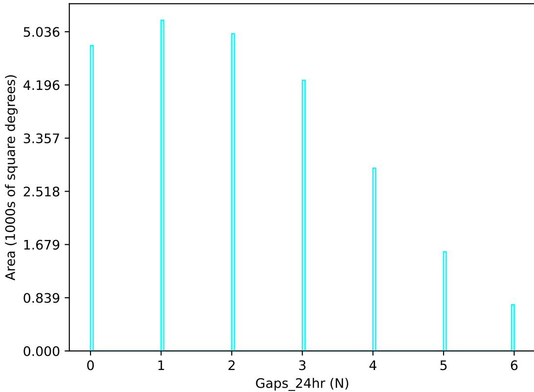
baseline_v2.1_10yrs u band: Gaps_24hr
