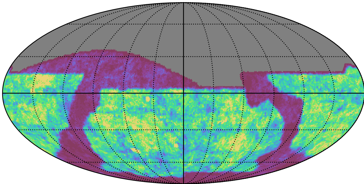
baseline_v2.1_10yrs r band: Gaps_24hr
