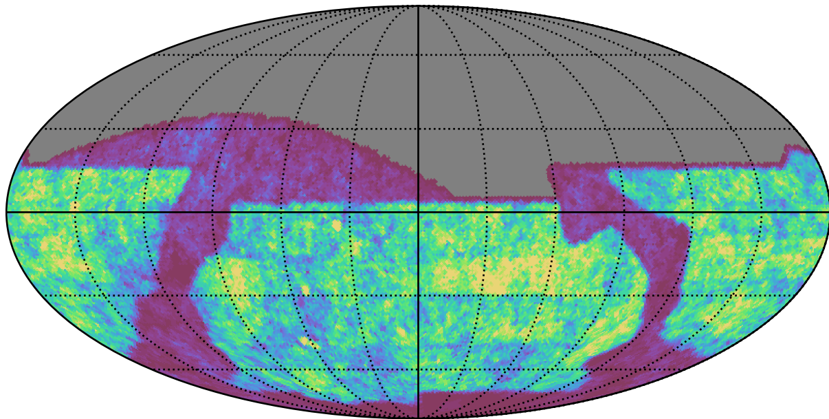
baseline_v2.1_10yrs i band: Gaps_24hr
