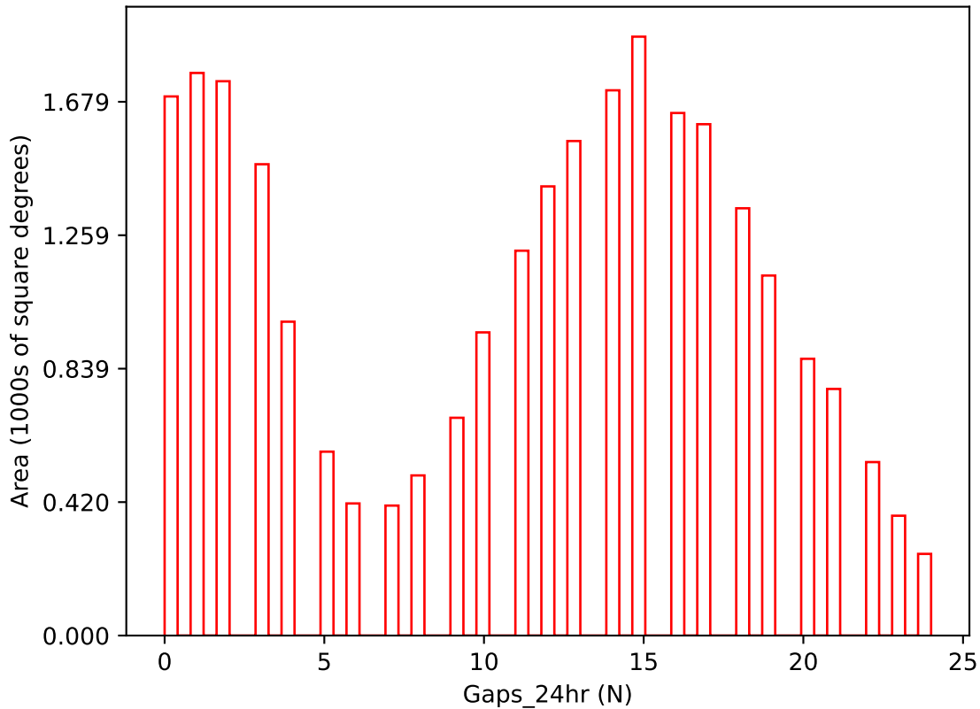
baseline_v2.1_10yrs i band: Gaps_24hr
