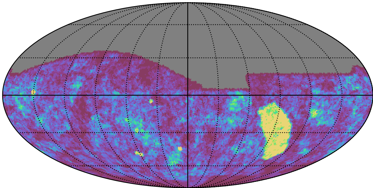
baseline_v2.1_10yrs g band: Gaps_24hr
