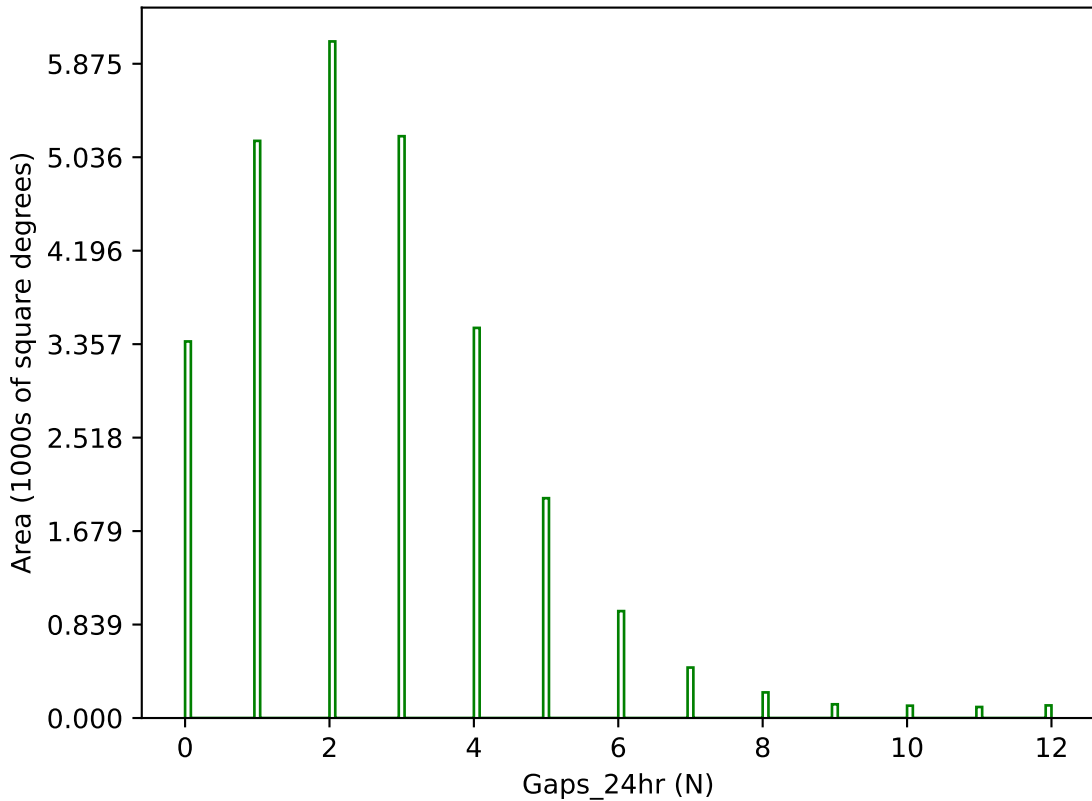
baseline_v2.1_10yrs g band: Gaps_24hr
