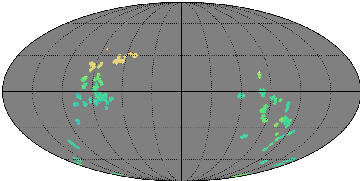
baseline_v2.1_10yrs : GalplaneTimePerFilter_zucker_sfr_map_z
